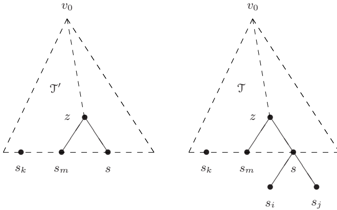
Fig. 10.7. Constructing (\mathcal{T}, w; v_0) starting from (\mathcal{T}', w'; v_0) .
