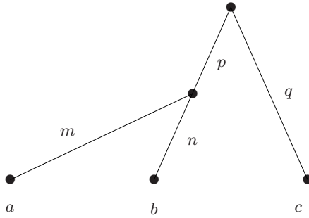
Fig. 10.3. Weighted tree.
