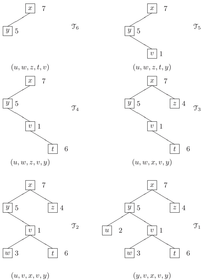
Fig. 3.22. Numbered trees with sequences (x_1, \dots, x_{i-1}, y_i, \dots, y_{n-1}) .
