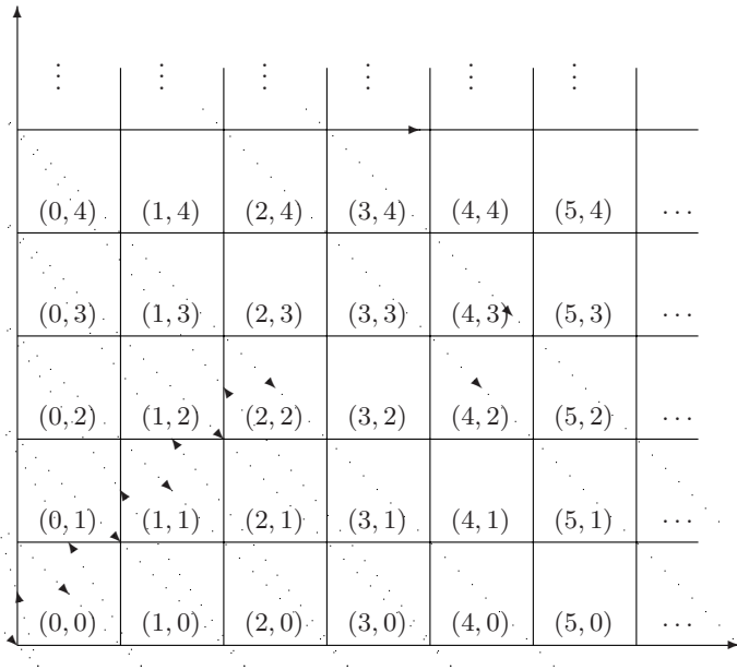
Fig. 1.2. Representation of \mathbb{N} \times \mathbb{N} .
