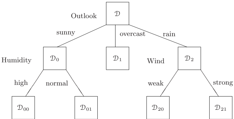
Fig. 9.2. Decision tree.
