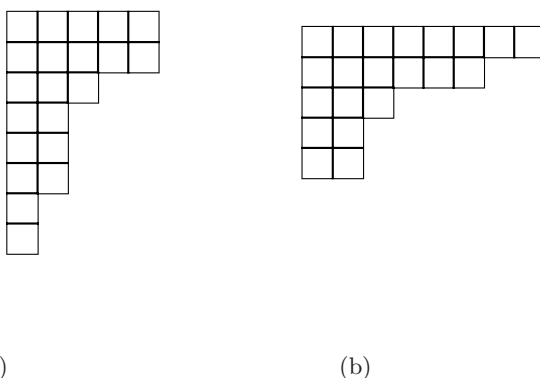
Fig. 14.1. Ferrers diagrams.
